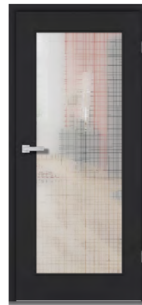
7 NORMTÜR NT-LA2-DA G-TEC® Schwarz Matt 9005 PANNO, Siebdruck-Veredelung KR1 CUBO, Edelstahl Matt MODEL STANDARD DOOR NT-LA2-DA FINISH G-TEC® Matte Black 9005 GLASS PANNO, screen printed décor FRAME KR1 FITTINGS CUBO, Stainless steel matt
